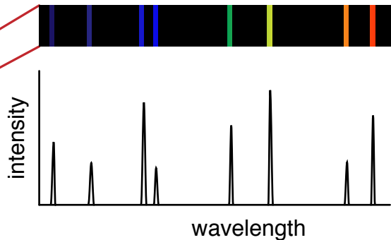
emission spectrum
