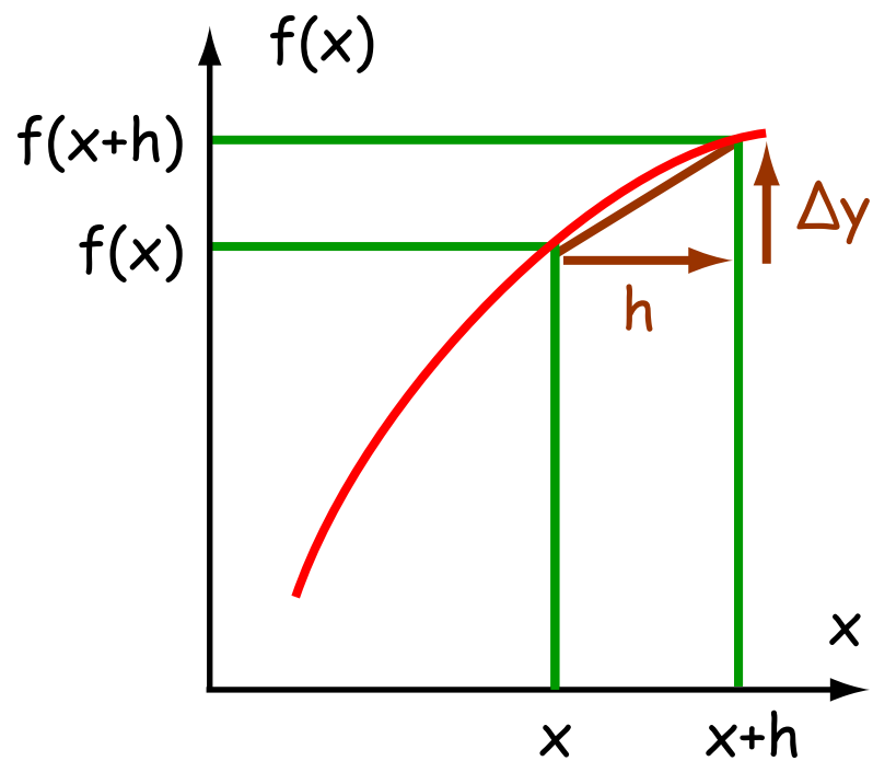
Forward difference derivative = \Delta y/h
