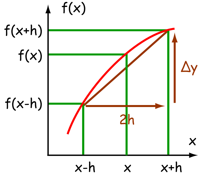
Symmetric difference derivative = \Delta y/2h
