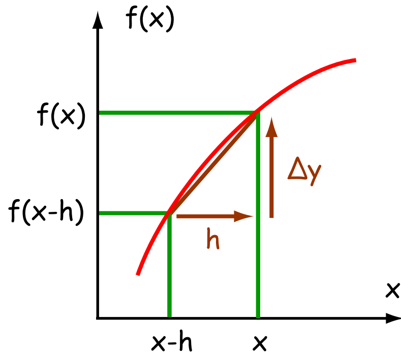
Backward difference derivative = \Delta y/h
