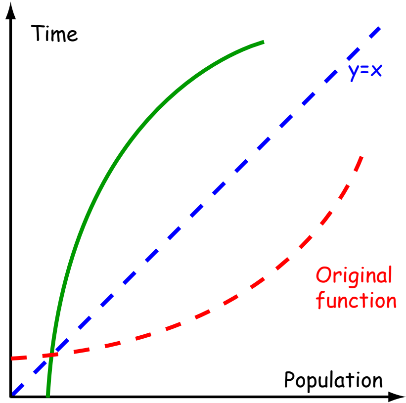
Inverse function
