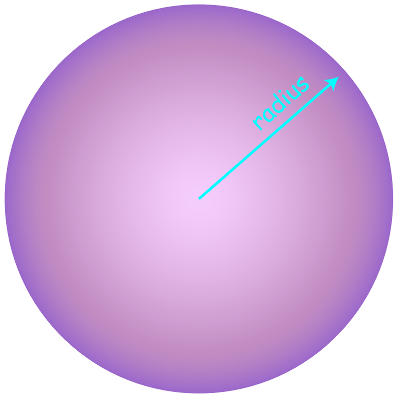
Circle on Plane Area = \pi r^2
