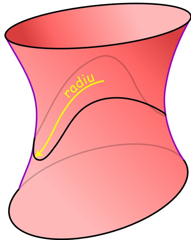
Circle on Hyperboloid Area < \pi r^2
