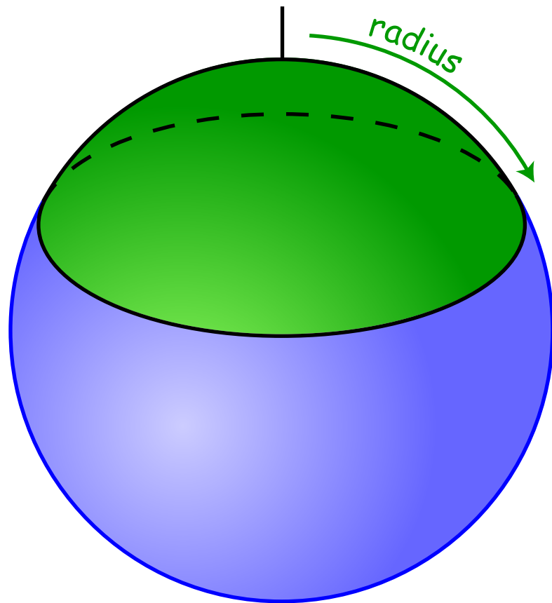
Circle on Sphere Area > \pi r^2
