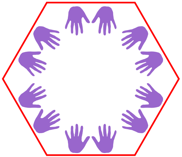
Lattice unit
