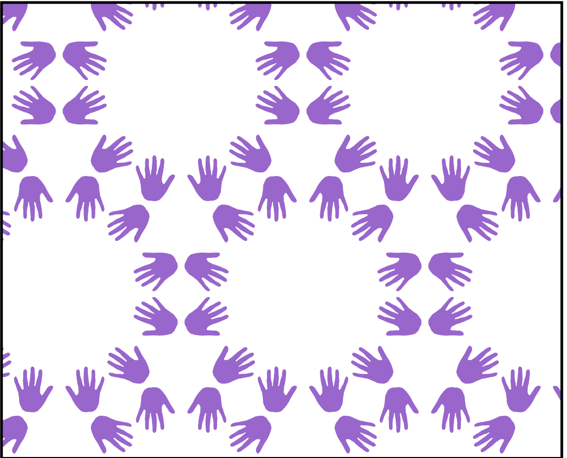
P6M Wallpaper
