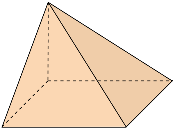
Skew square pyramid
