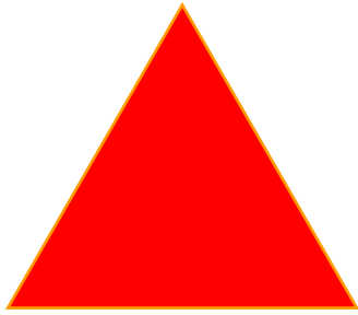
Regular Triangle
