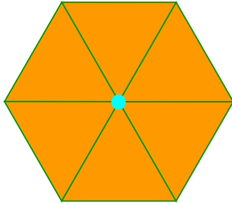
Base Tile: 3.3.3.3.3.3
