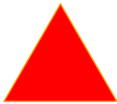
Regular Triangle
