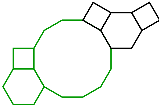
Tile Piece
