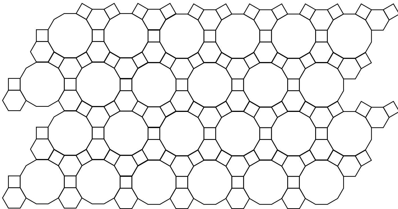
Tessellation
