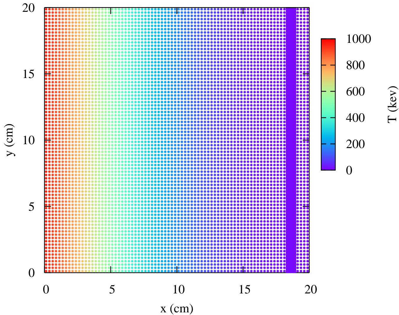
Material Temperature, Su-Olson on 200x200 uniform mesh at t=0.1 sh
