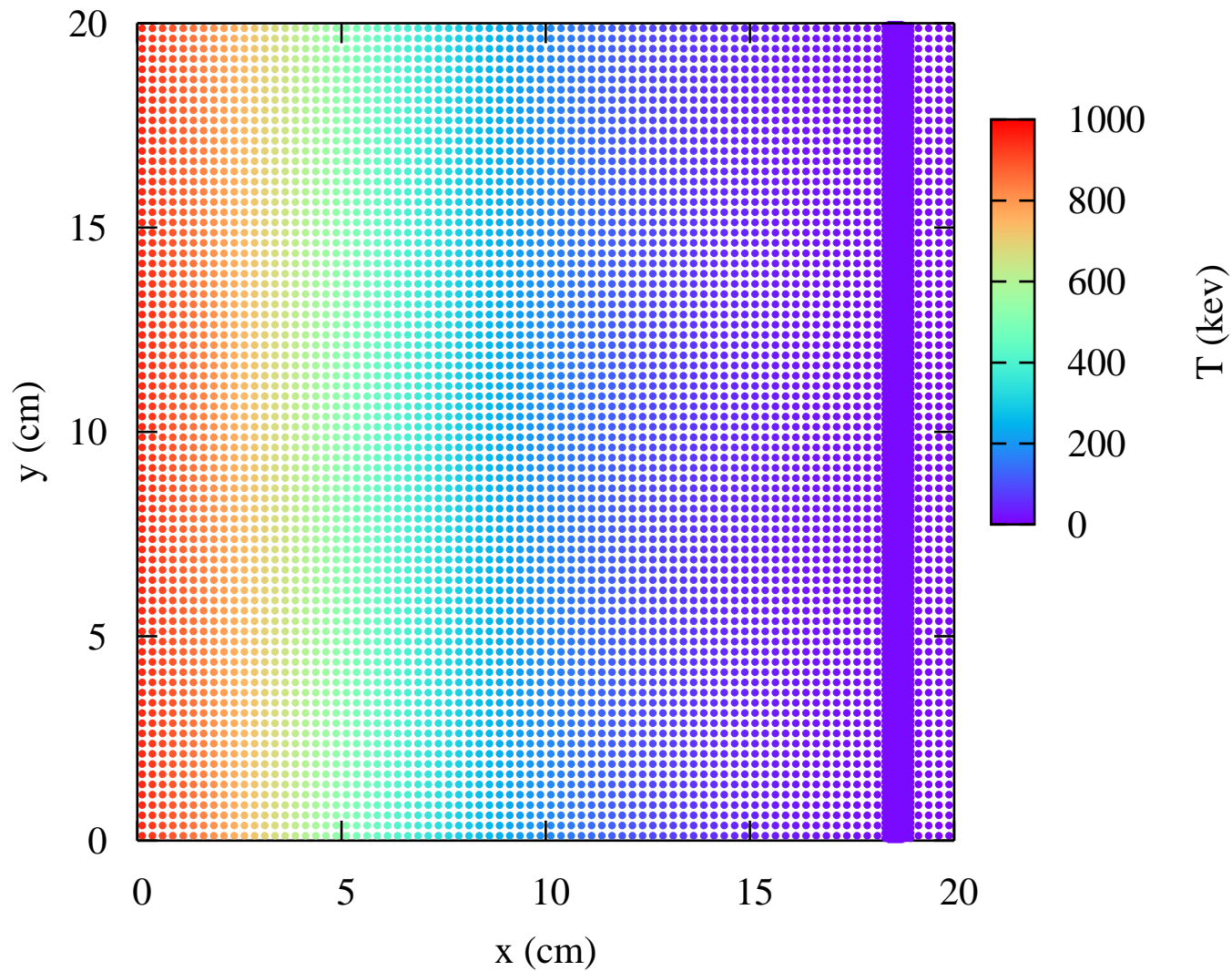
Material Temperature, Su-Olson on 400x400 uniform mesh at t=0.1 sh
