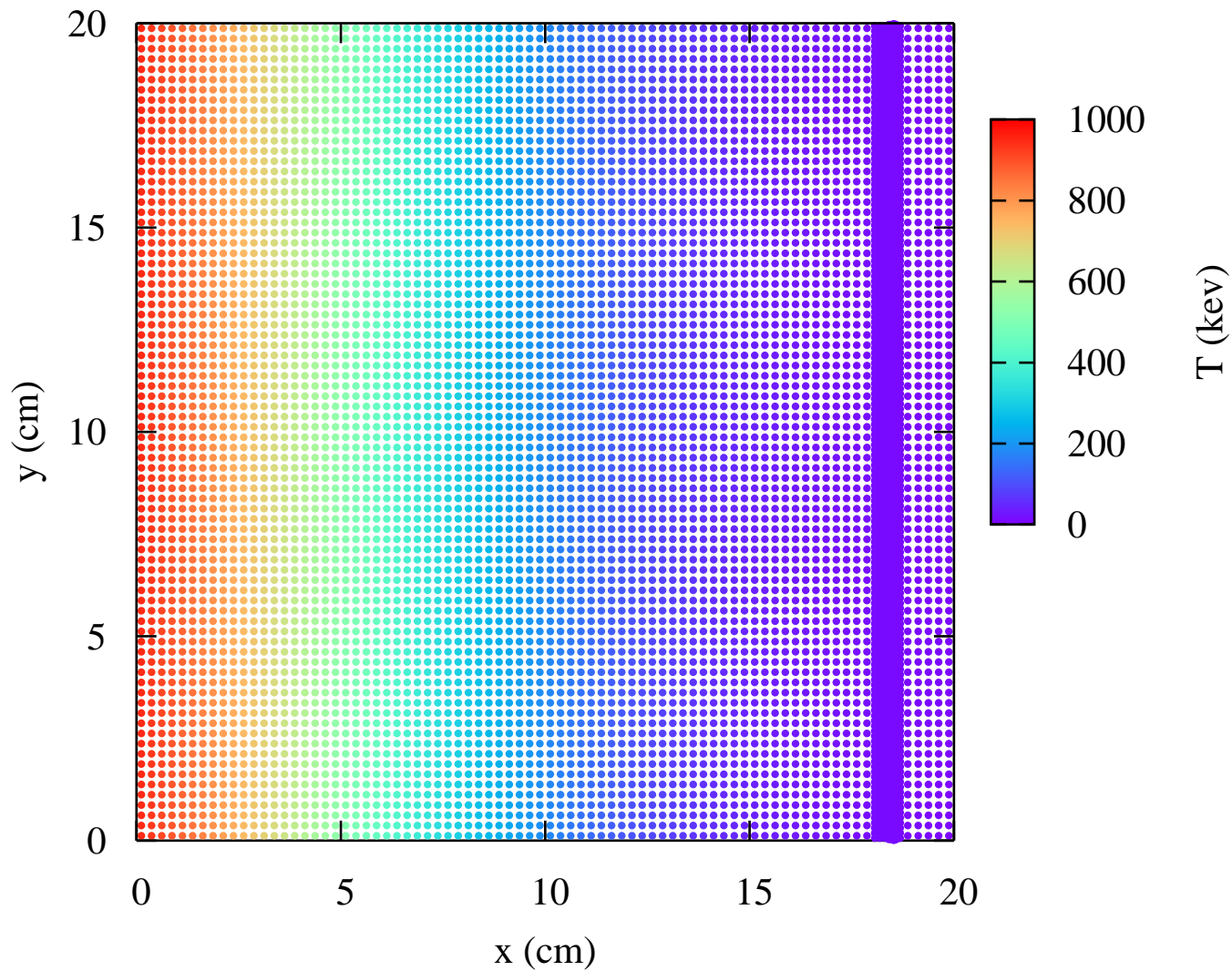
Material Temperature, Su-Olson on 800x800 uniform mesh at t=0.1 sh
