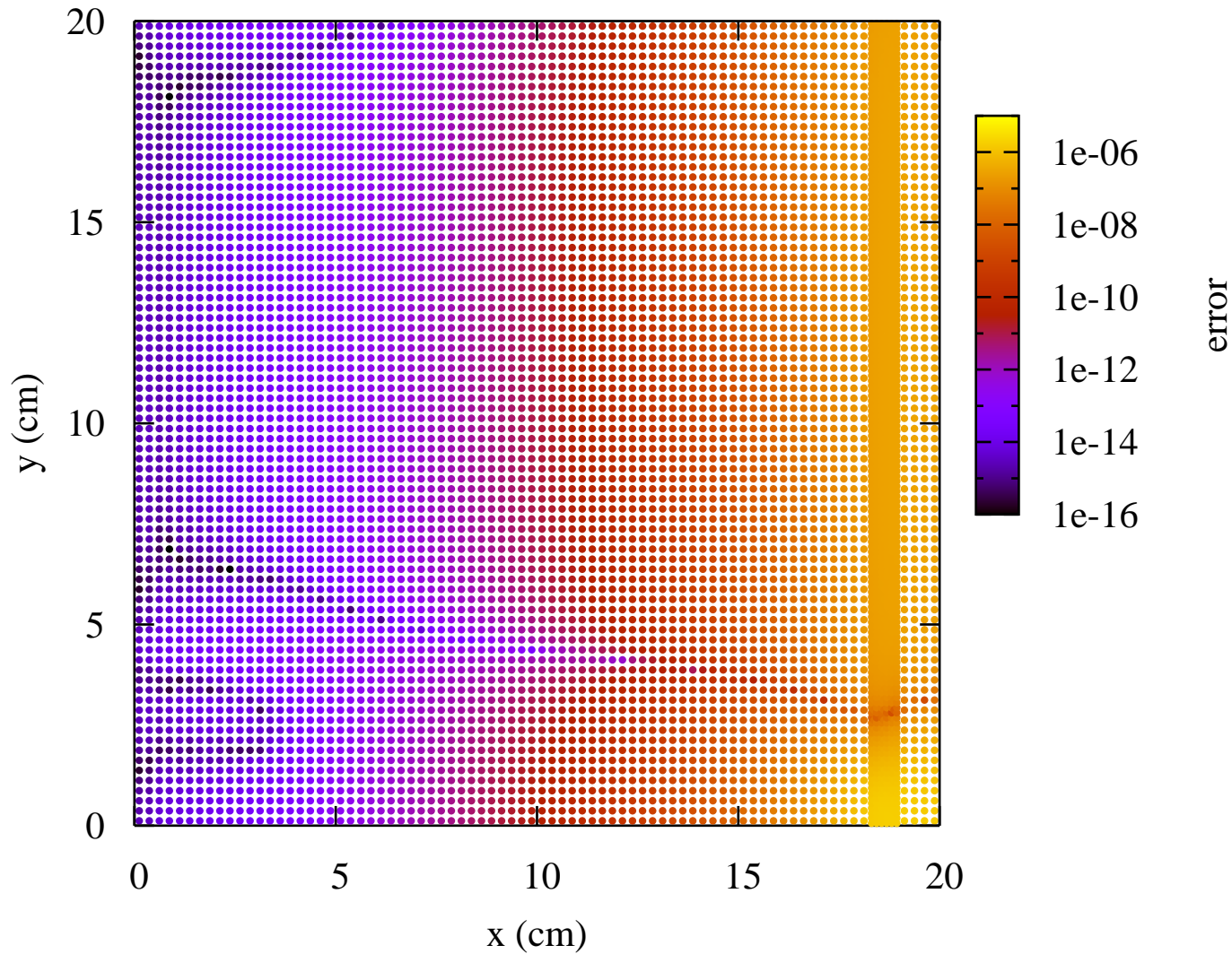
Su-Olson: asymmetry in material temperature, 200x200 uniform mesh, t=0.1 sh
