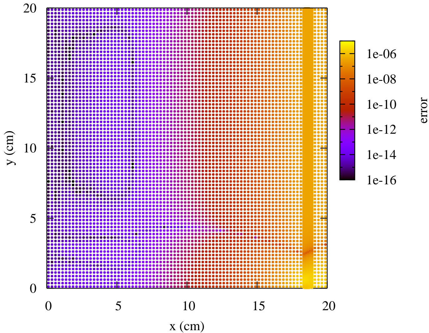
Su-Olson: asymmetry in material temperature, 400x400 uniform mesh, t=0.1 sh
