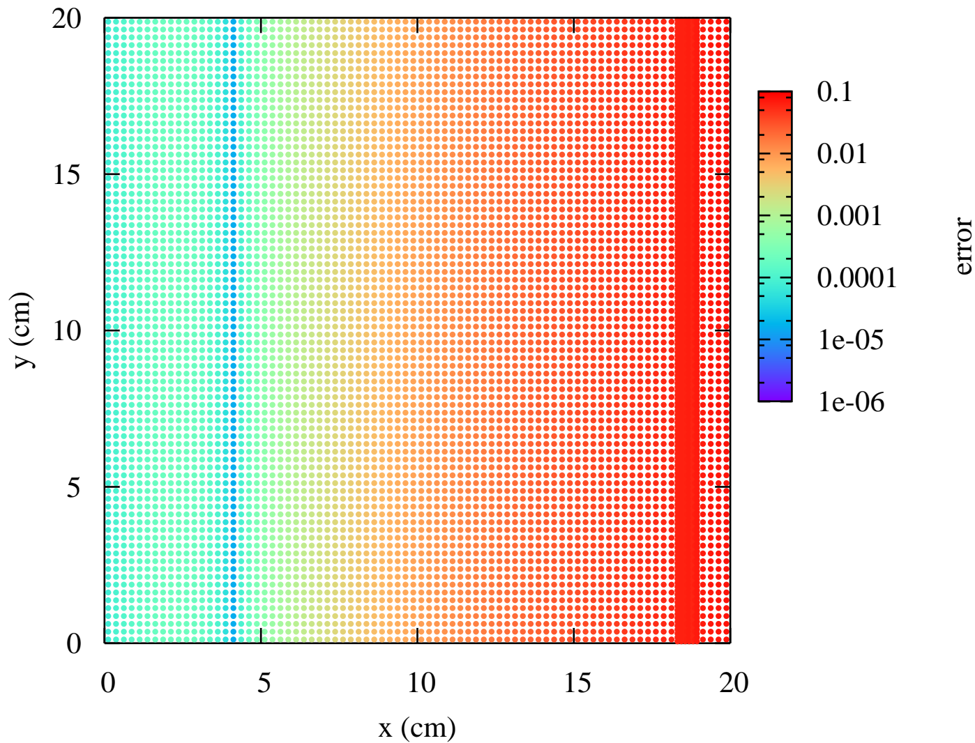
Su-Olson: error in radiation temperature, 200x200 uniform mesh, t=0.1 sh
