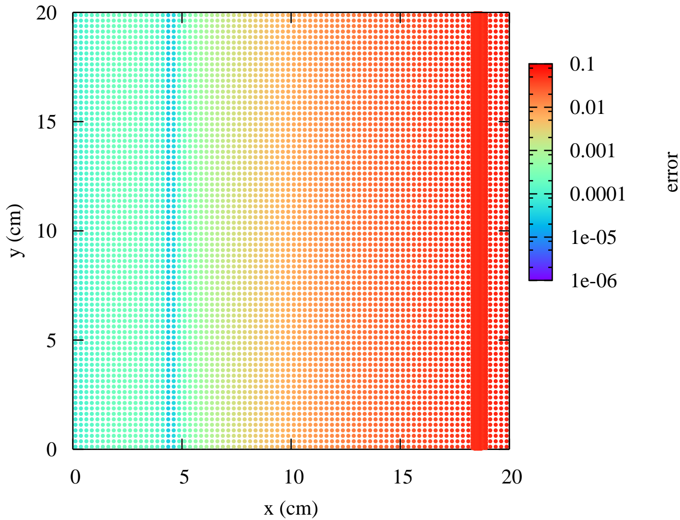
Su-Olson: error in radiation temperature, 400x400 uniform mesh, t=0.1 sh
