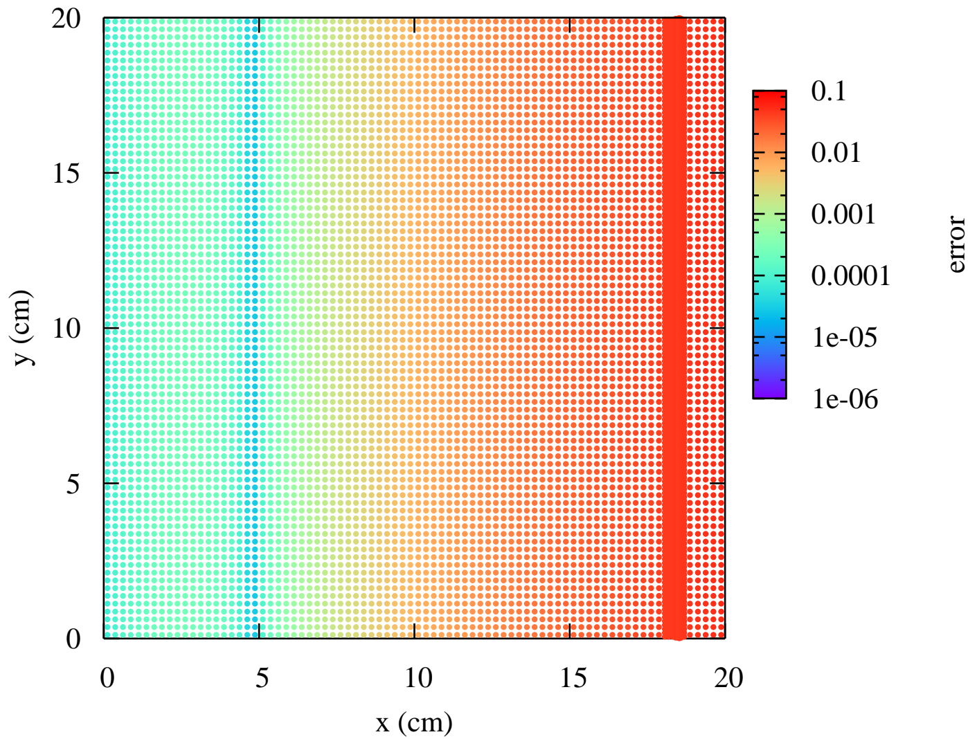
Su-Olson: error in radiation temperature, 800x800 uniform mesh, t=0.1 sh
